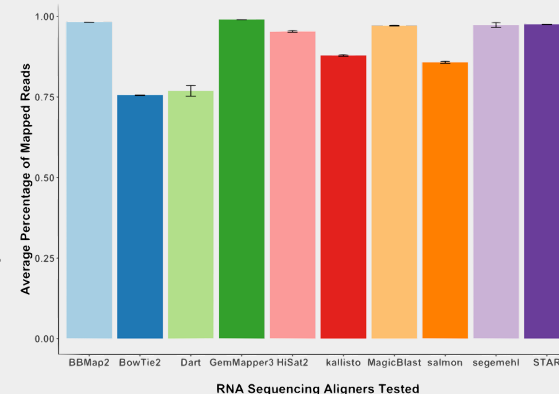
Figure 3: Percentage of Mapped Reads for the Aligners with Default Settings (averaged across RNAseq samples)
