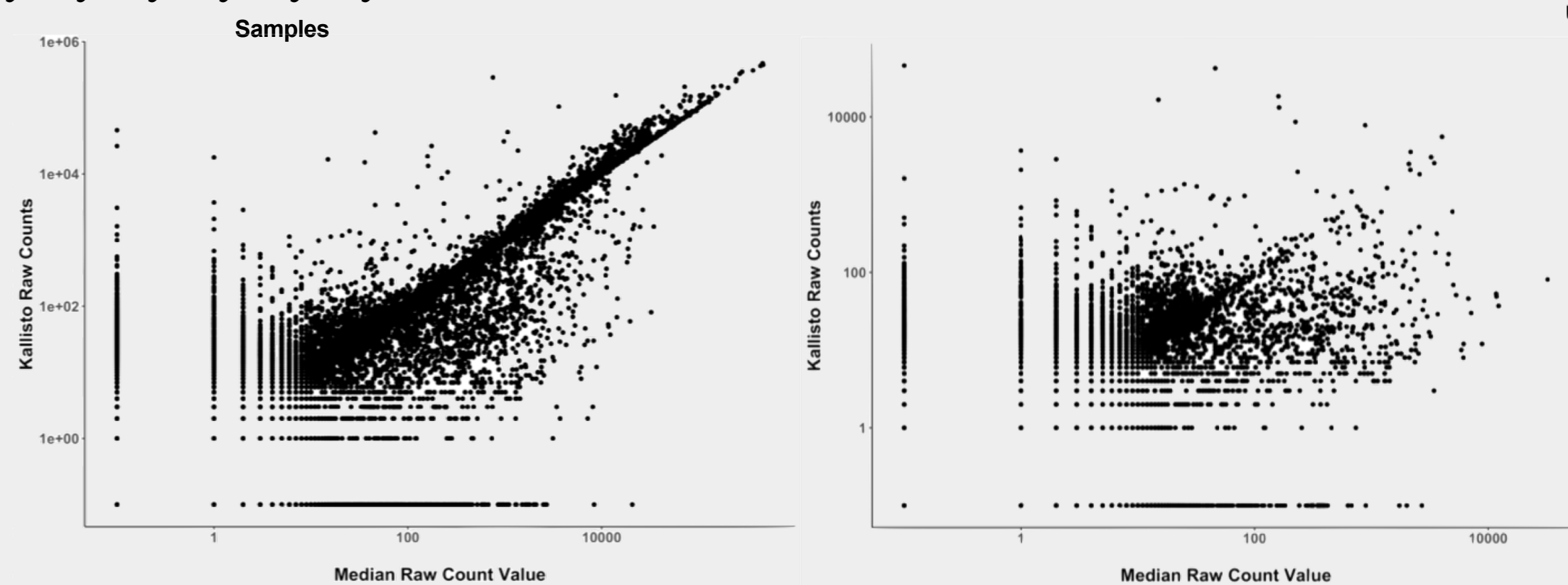
Figure 7: Alignment profiles comparing Kallisto pseudoalignment (y-axis) and the median across ten aligners (x-axis) for Detected (left) and Low-Expression (right) genes
