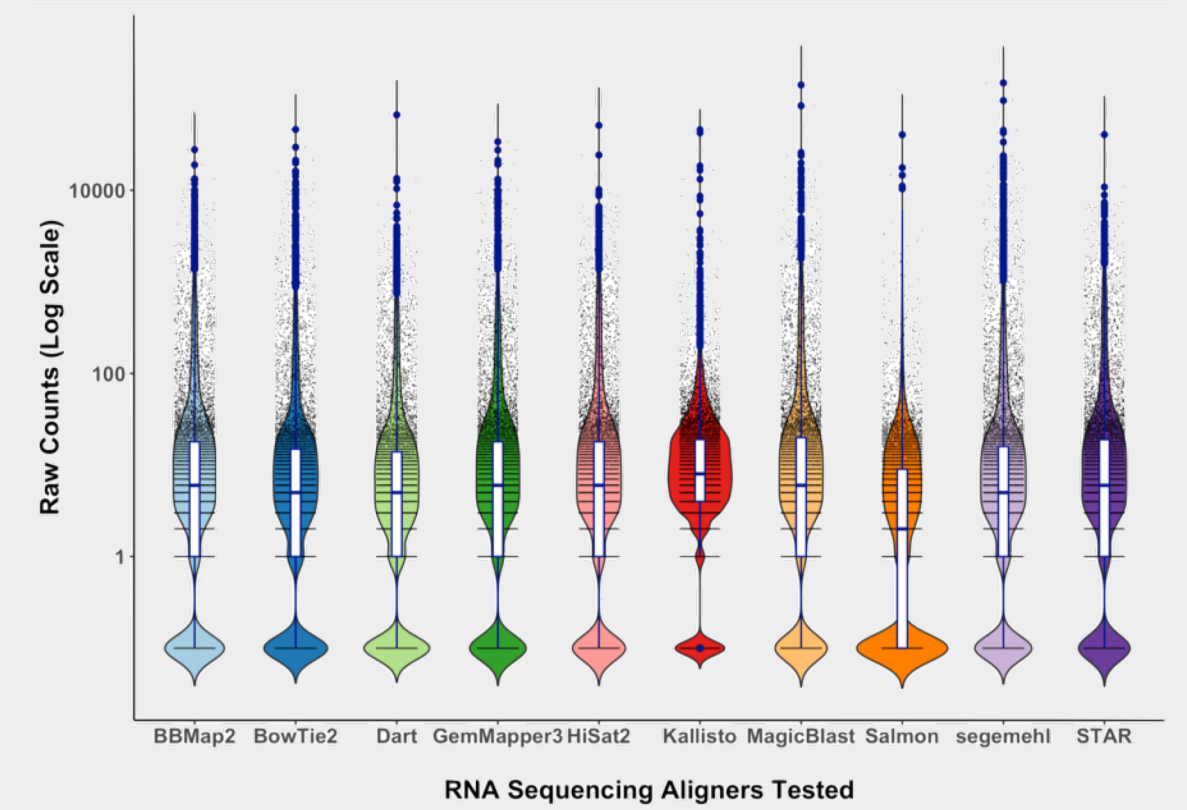
Figure 5: Distribution of Counts for Low-Expression Genes (raw value >= 22 >= value >= 3 for at least one aligner)
