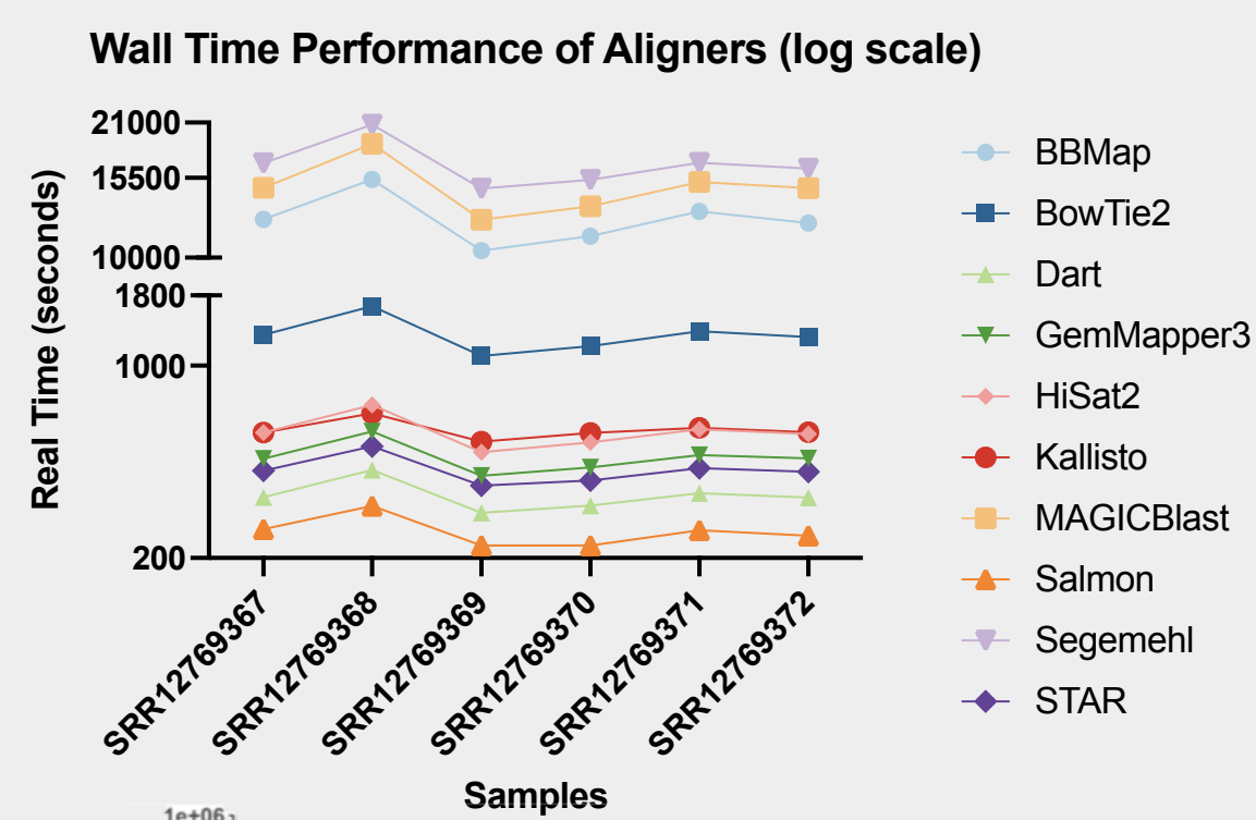
Figure 2: Wall Time Performance for the Aligners with Default Settings (split across six RNAseq samples)
